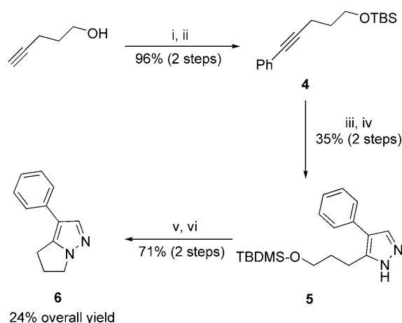
Scheme 5. Synthesis of withasomnine ( 6 ). (i) 1 mol% \text{Pd}(\text{PPh}_3)_4 , 2 mol% \text{CuI} , 2 equiv. \text{PhI} , 10 equiv. \text{NEt}_3 , THF. (ii) \text{ClSiMe}_2(t\text{-Bu}) , imidazole, DMF. (iii) \text{PhNH}_2 , t\text{-BuNC} , 10 mol% 2 , 110 °C, 48 h, toluene. (iv) \text{NH}_2\text{NH}_2 , pyridine, 150 °C, 24 h. (v) \text{BBr}_3 , \text{CH}_2\text{Cl}_2 , room temperature, 48 h. (vi) \text{NaOEt} , \text{HOEt} , reflux, 20 h.
